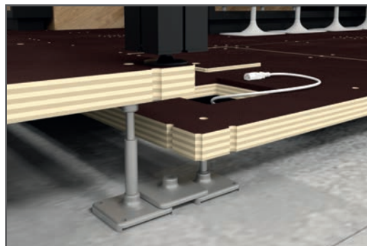
The double floor system OCTAfloor allows for the efficient laying of pipes and cables as well as platform construction.
